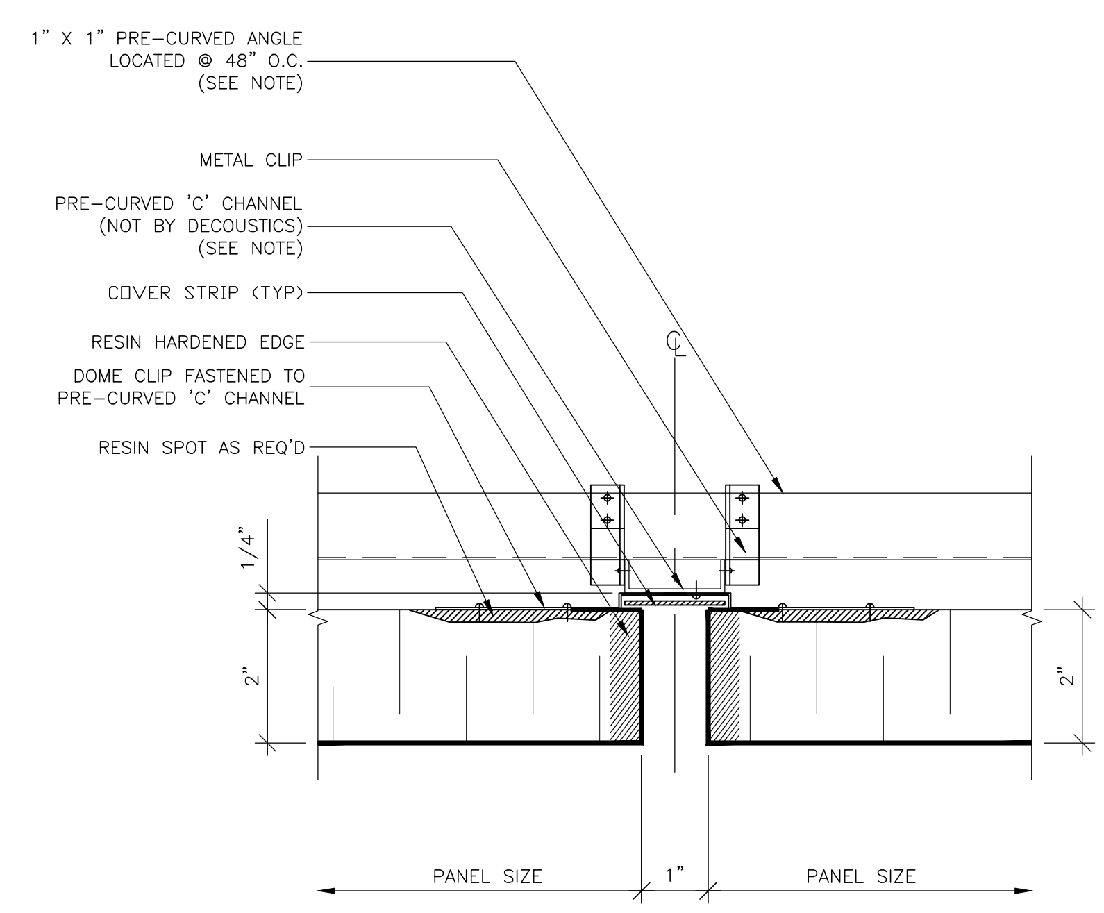
4 DOME CLIP VERTICAL JOINT DETAIL SCALE: 6" = 1'-0"
