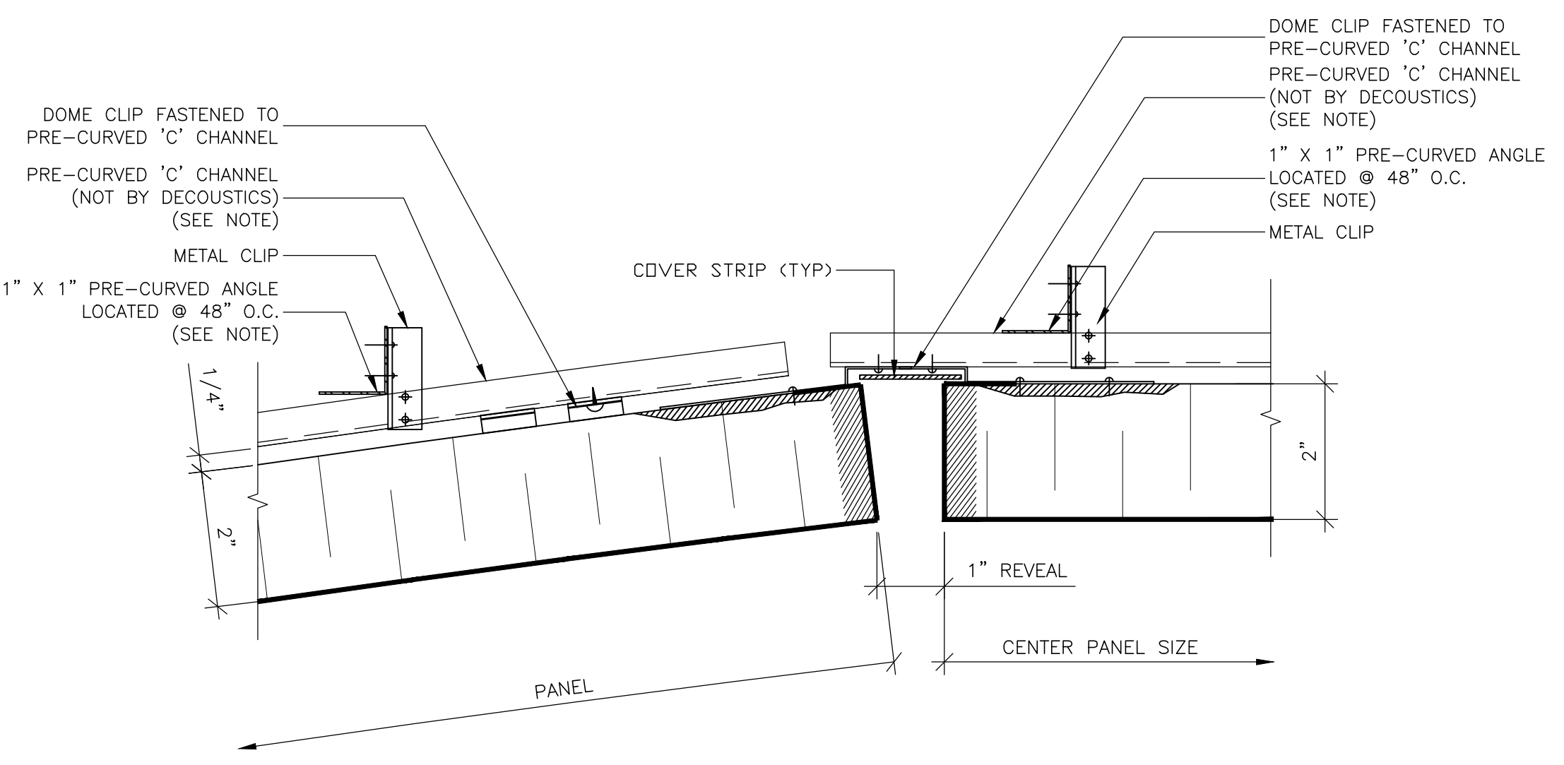
3 DOME CLIP JOINT DETAIL @ CENTER SCALE: 6" = 1'-0"
