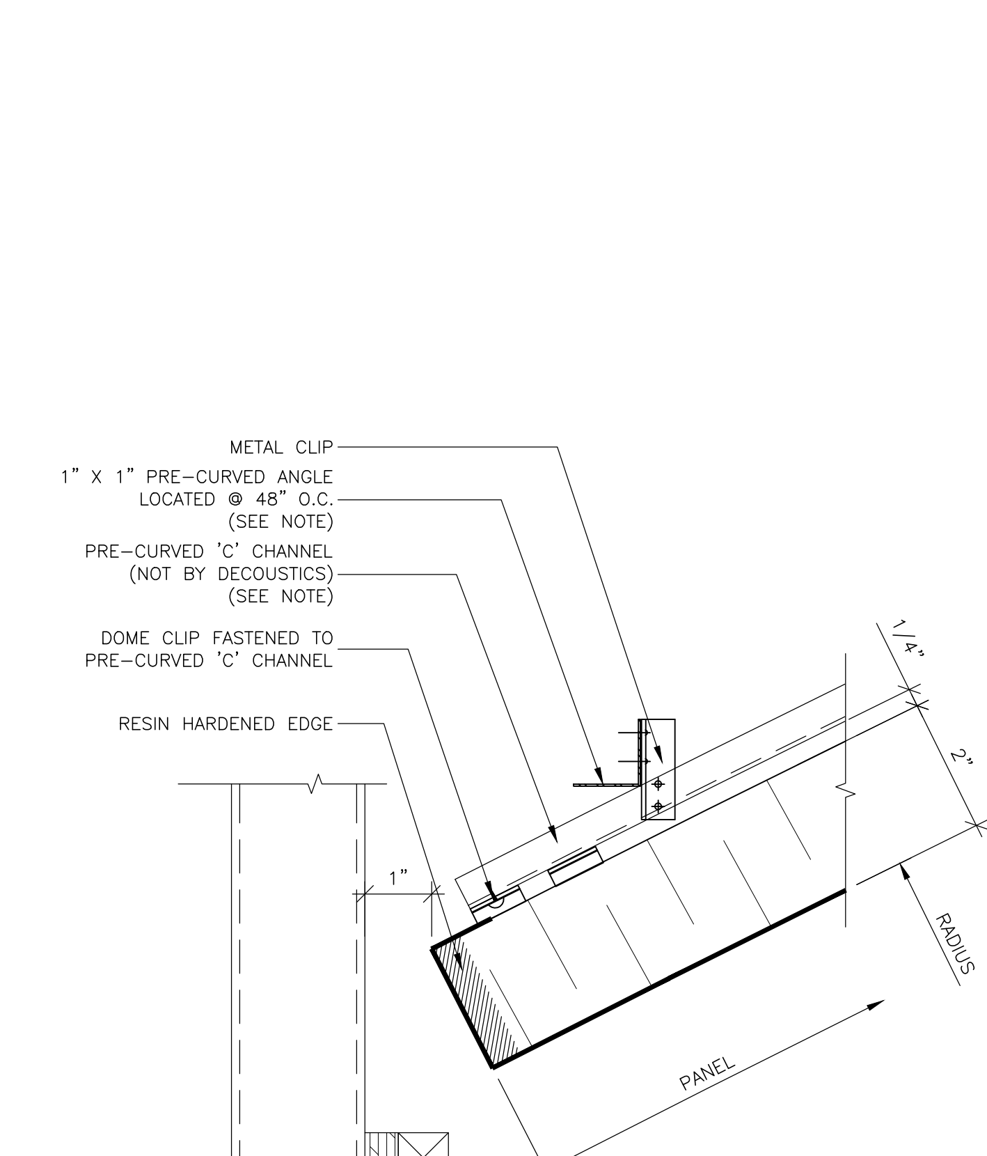
2 DOME CLIP JOINT DETAIL SCALE: 6" = 1'-0"
