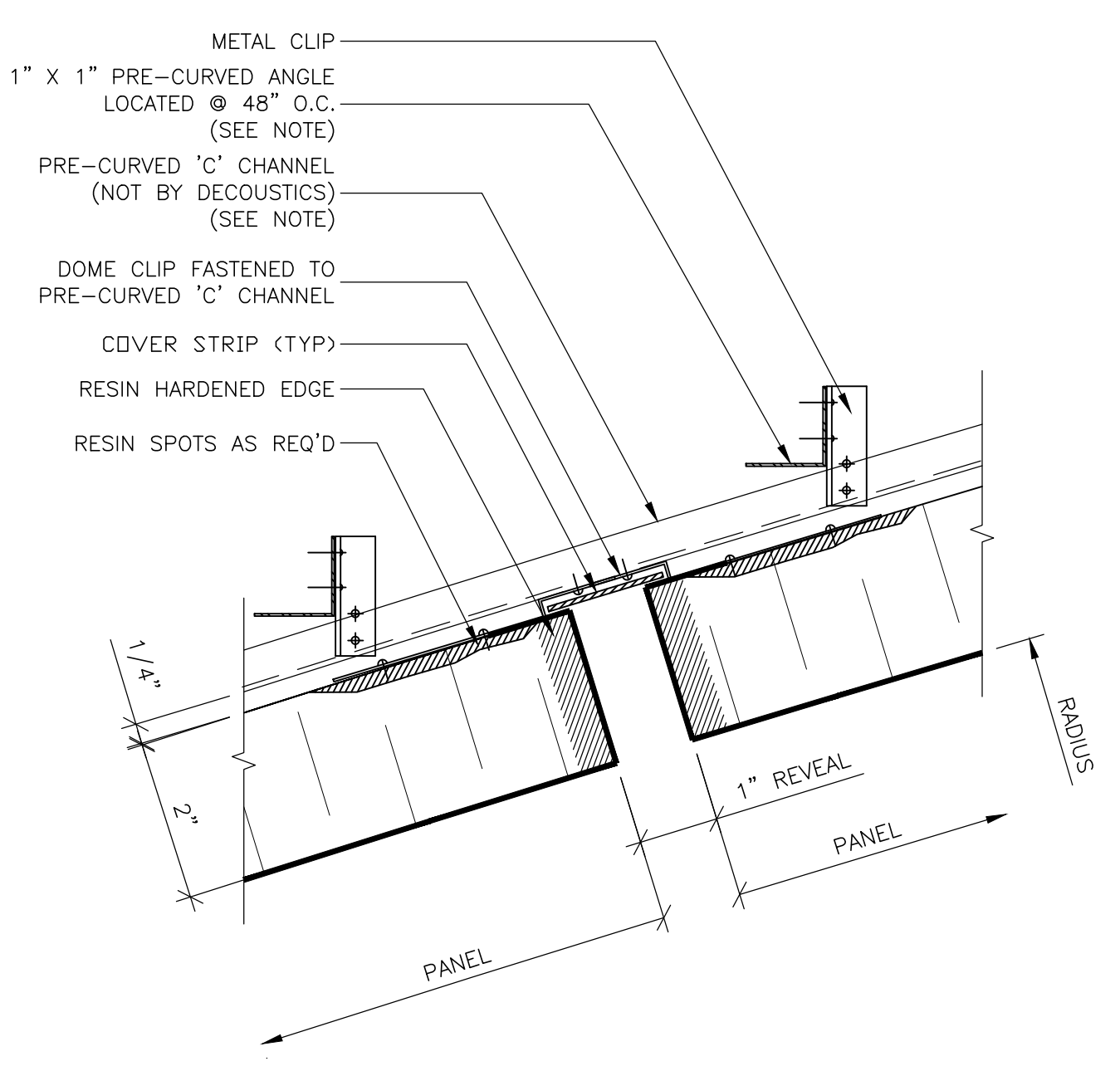
2 DOME CLIP JOINT DETAIL SCALE: 6" = 1'-0"
