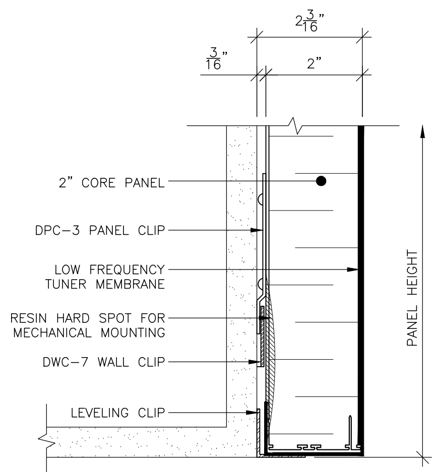
5 PANEL BASE @ BULKHEAD SCALE: 6" = 1'-0" REF: D1
