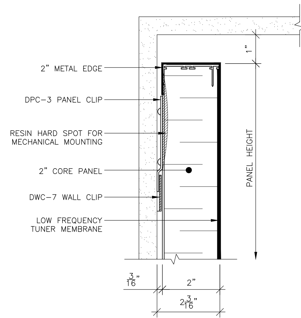
2 PANEL HEAD @ BULKHEAD SCALE: 6" = 1'-0" REF: D1
