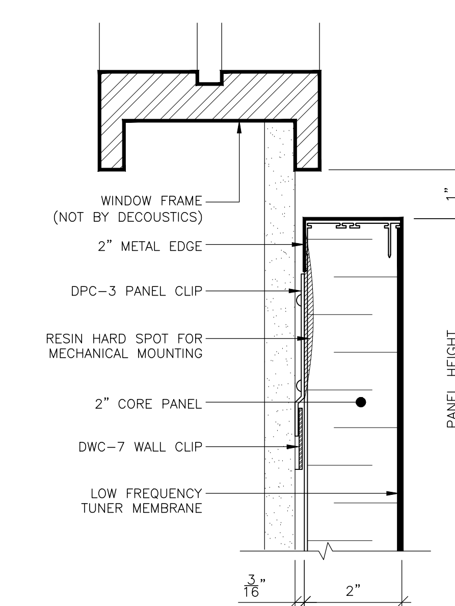
12 PANEL HEAD @ FRAME SCALE: 6" = 1'-0" REF: D1
