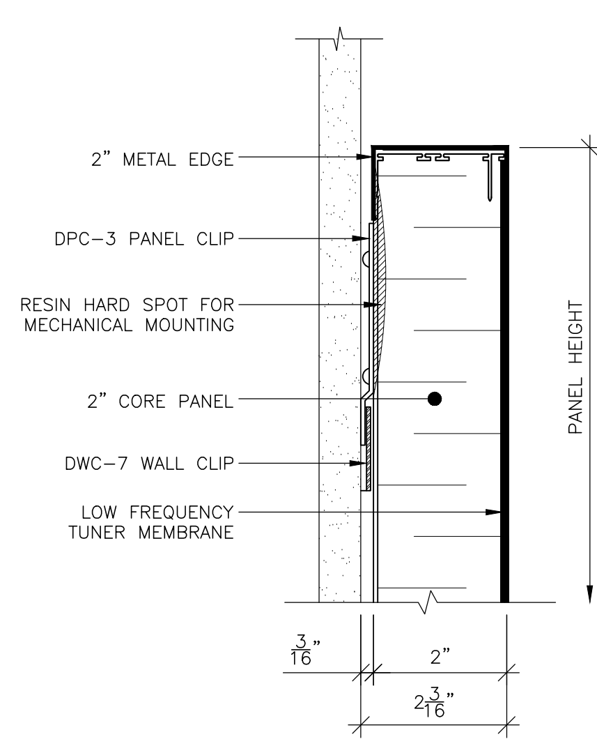
1 PANEL HEAD @ WALL SCALE: 6" = 1'-0" REF: D1
