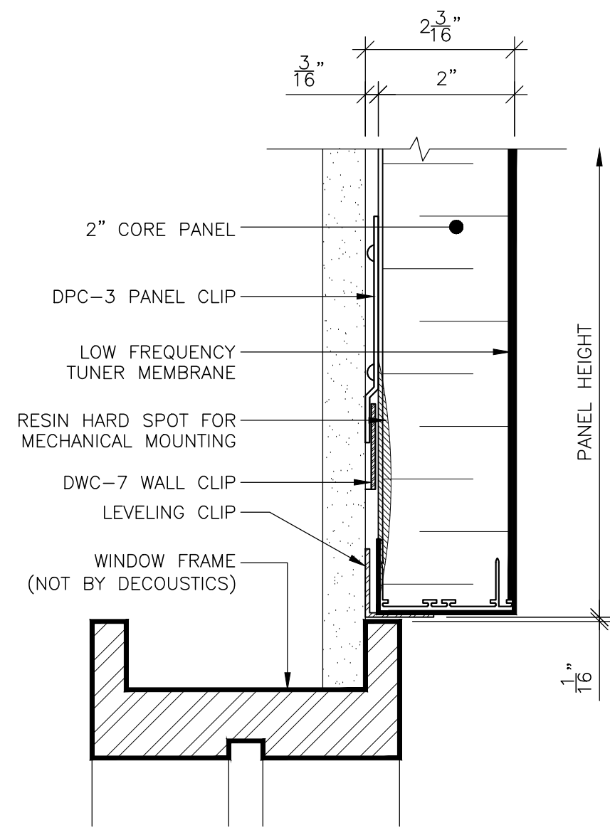
1 PANEL BASE @ FRAME D2 SCALE: 6" = 1'-0" REF:
