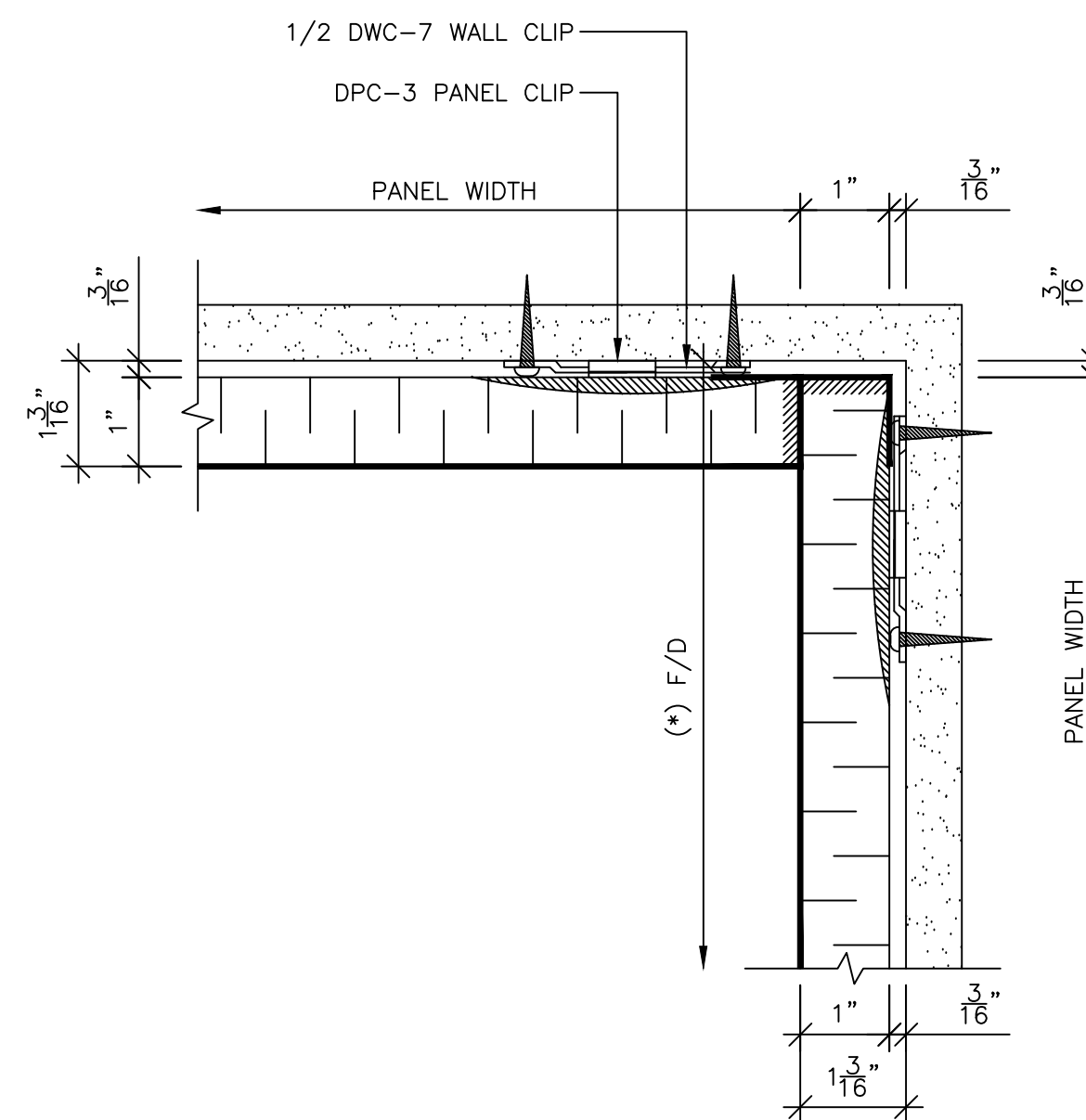
7 PANEL END @ CORNER SCALE: 6" = 1'-0" REF:
