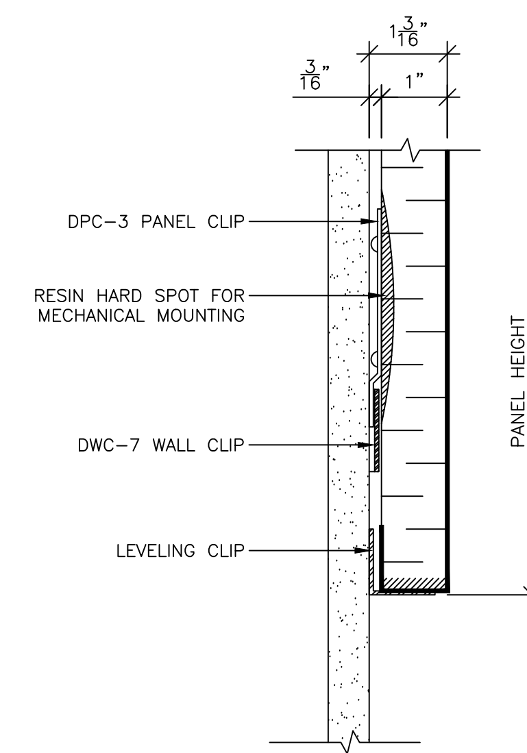
6 PANEL BASE @ WALL SCALE: 6" = 1'-0" REF:
