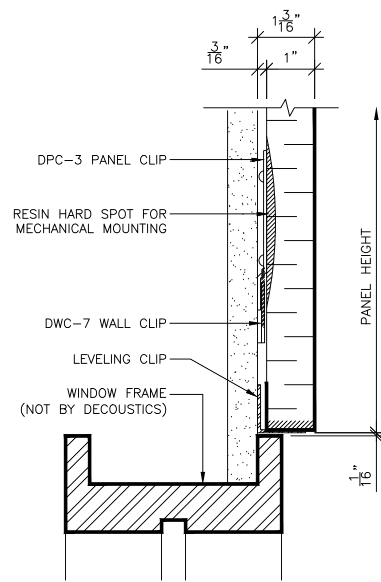
1 PANEL BASE @ FRAME D2 SCALE: 6" = 1'-0" REF:
