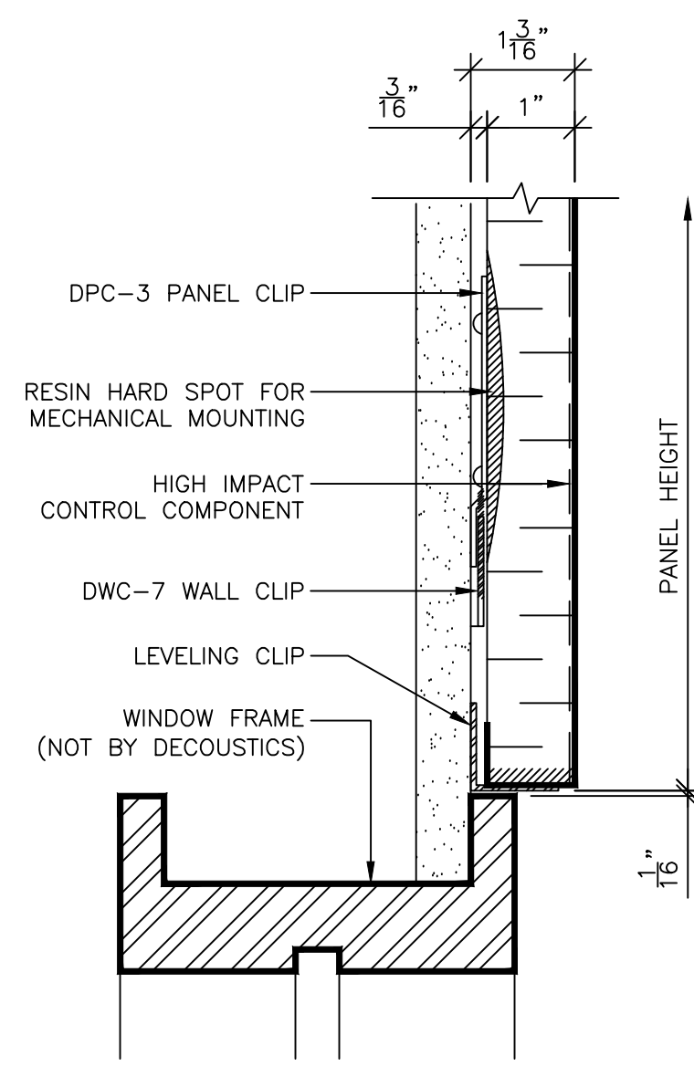
1 PANEL BASE @ FRAME SCALE: 6" = 1'-0" REF:
