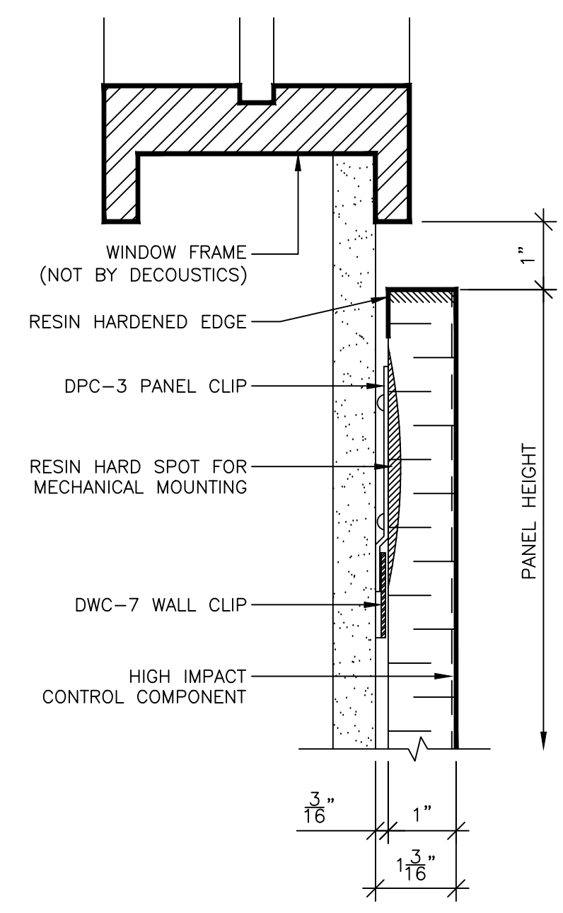
12 PANEL HEAD @ FRAME SCALE: 6" = 1'-0" REF:
