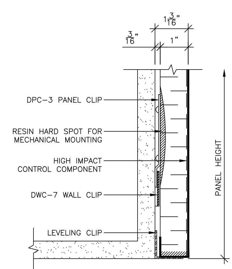
5 PANEL BASE @ BULKHEAD SCALE: 6" = 1'-0" REF:
