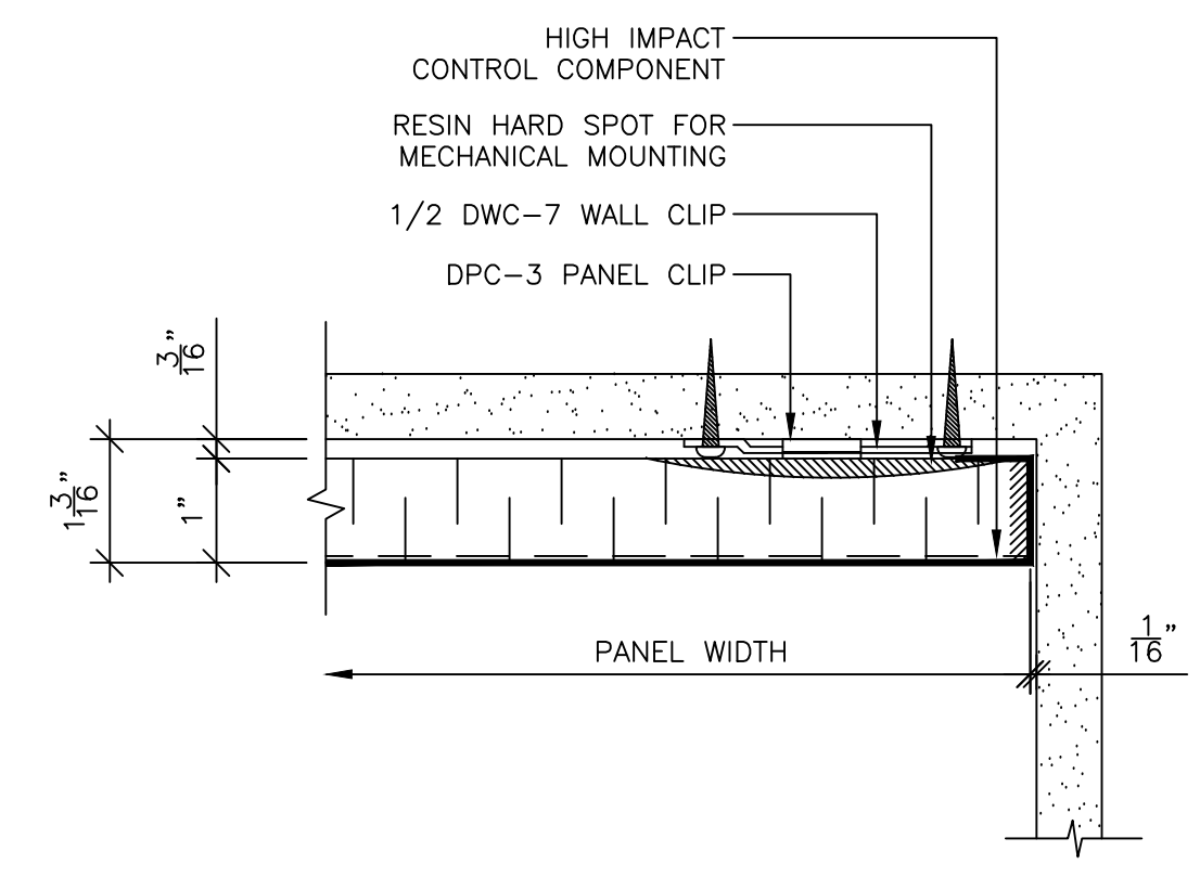
8 PANEL END @ WALL SCALE: 6" = 1'-0" REF:
