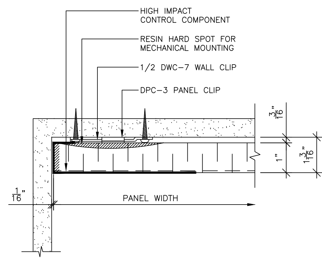
3 PANEL END @ WALL SCALE: 6" = 1'-0" REF:
