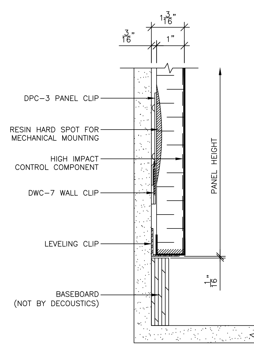
2 PANEL BASE @ BASEBOARD SCALE: 6" = 1'-0" REF:
