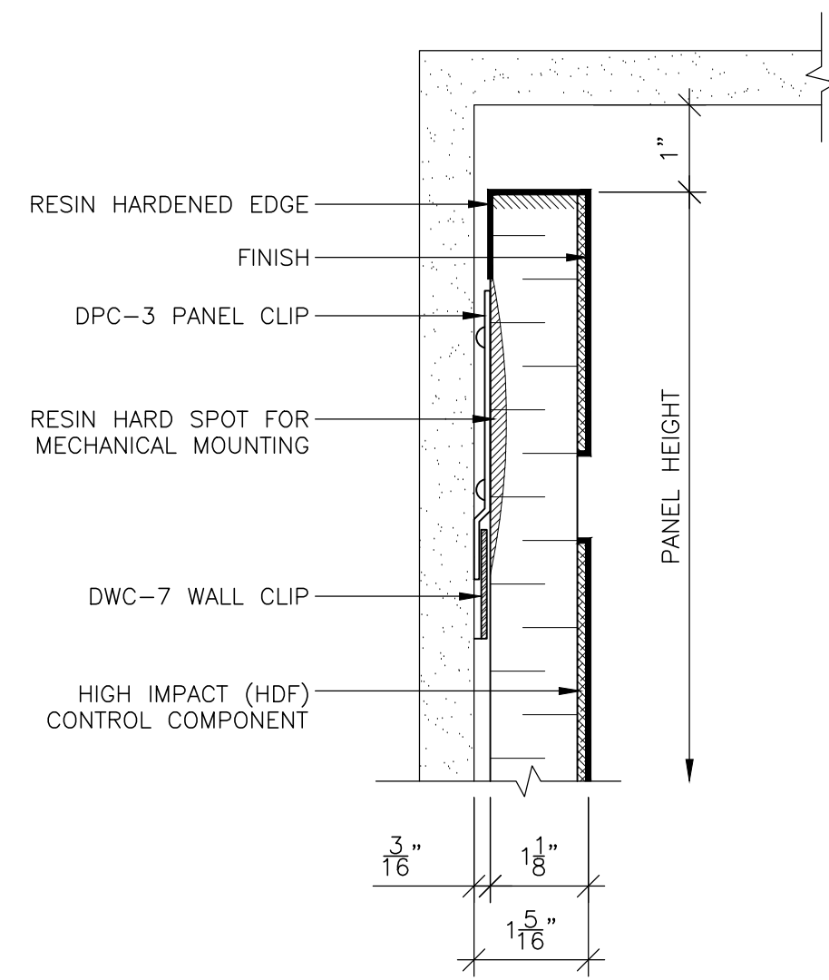
2 PANEL HEAD @ BULKHEAD SCALE: 6" = 1'-0" REF: D1
