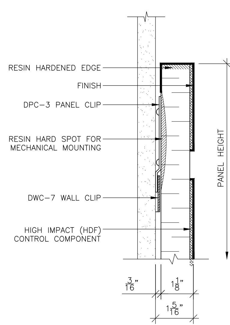
1 PANEL HEAD @ WALL SCALE: 6" = 1'-0" REF: D1
