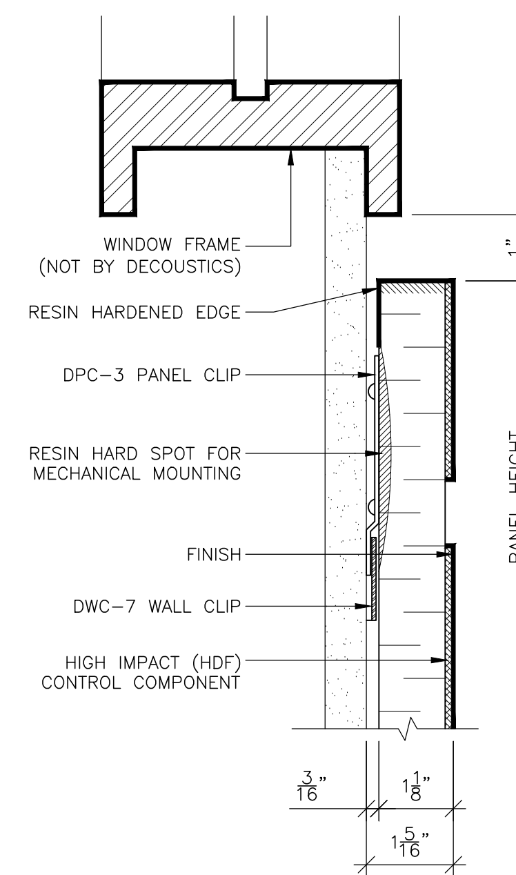
12 PANEL HEAD @ FRAME SCALE: 6" = 1'-0" REF: D1
