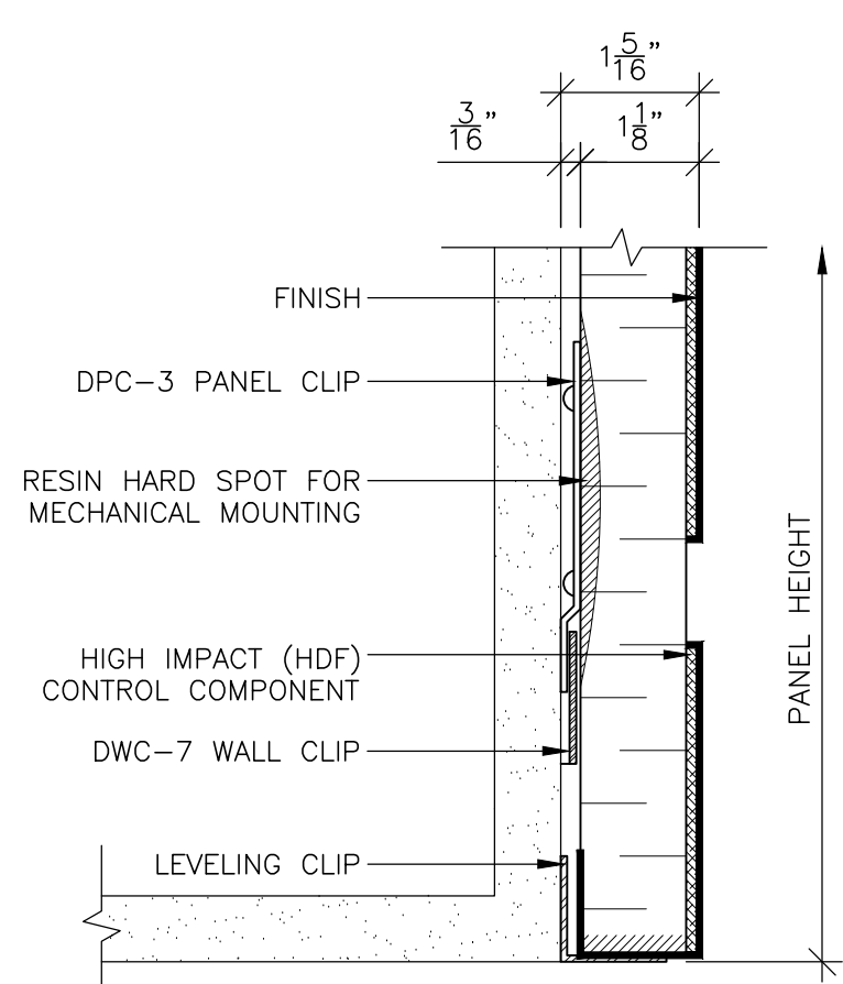
5 PANEL BASE @ BULKHEAD SCALE: 6" = 1'-0" REF: D1
