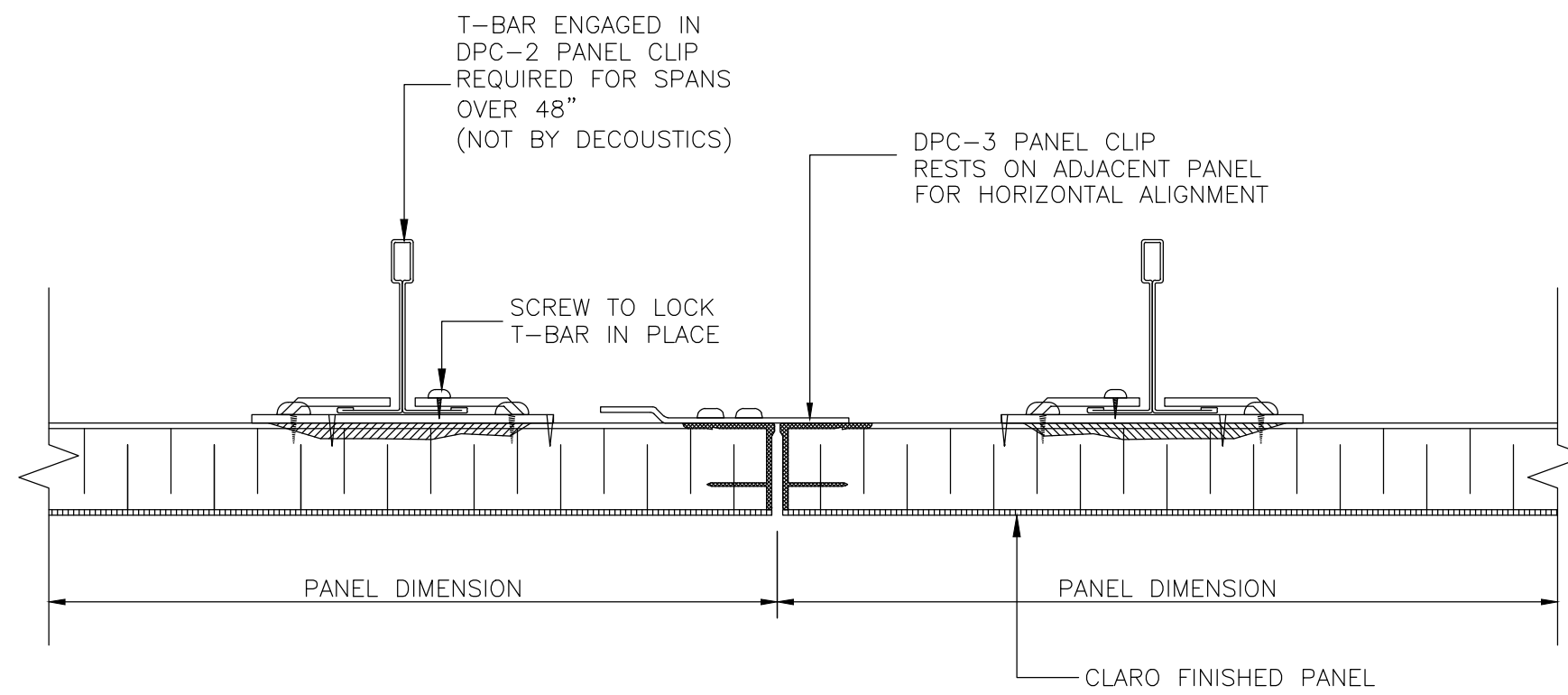
2 DETAIL @ PANEL'S JOINT D1 SCALE: 1/2"=1"
