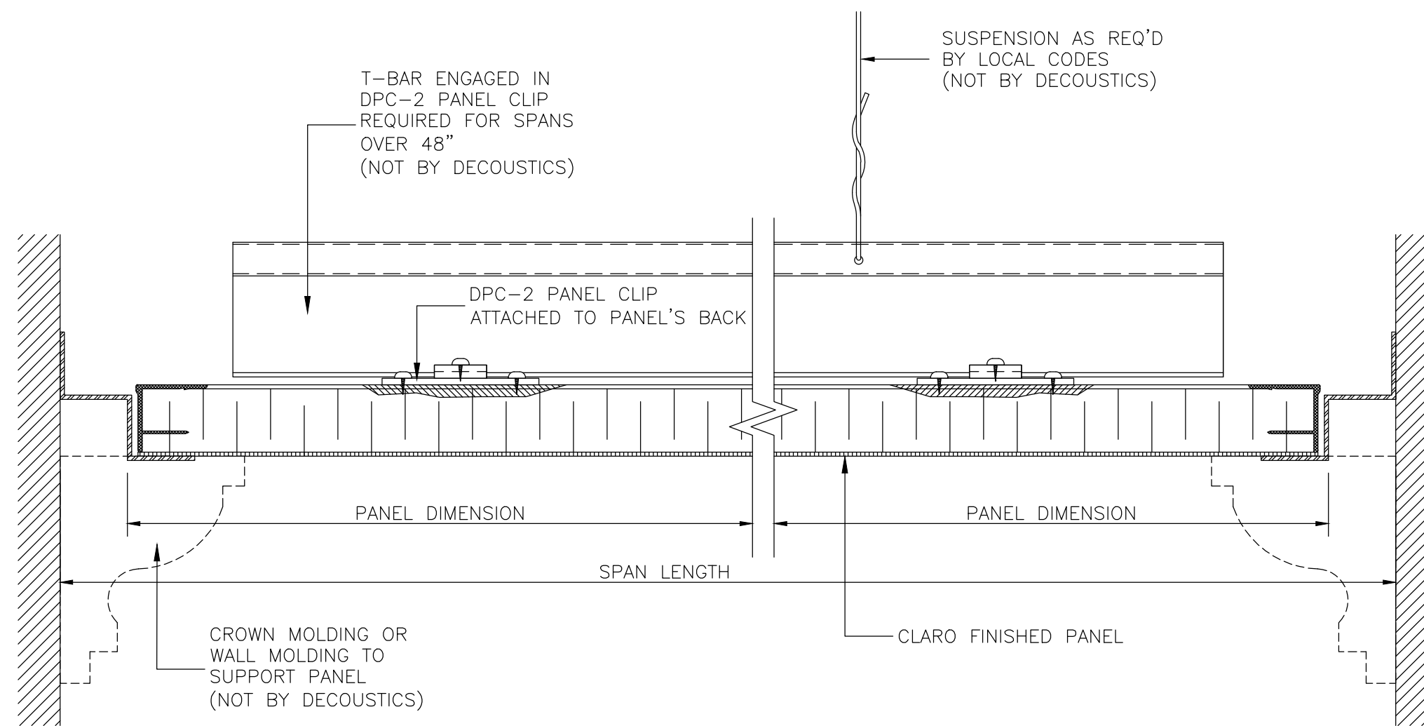
1 PANEL DETAIL @ SPAN LENGTH D1 SCALE: 1/2"=1"
