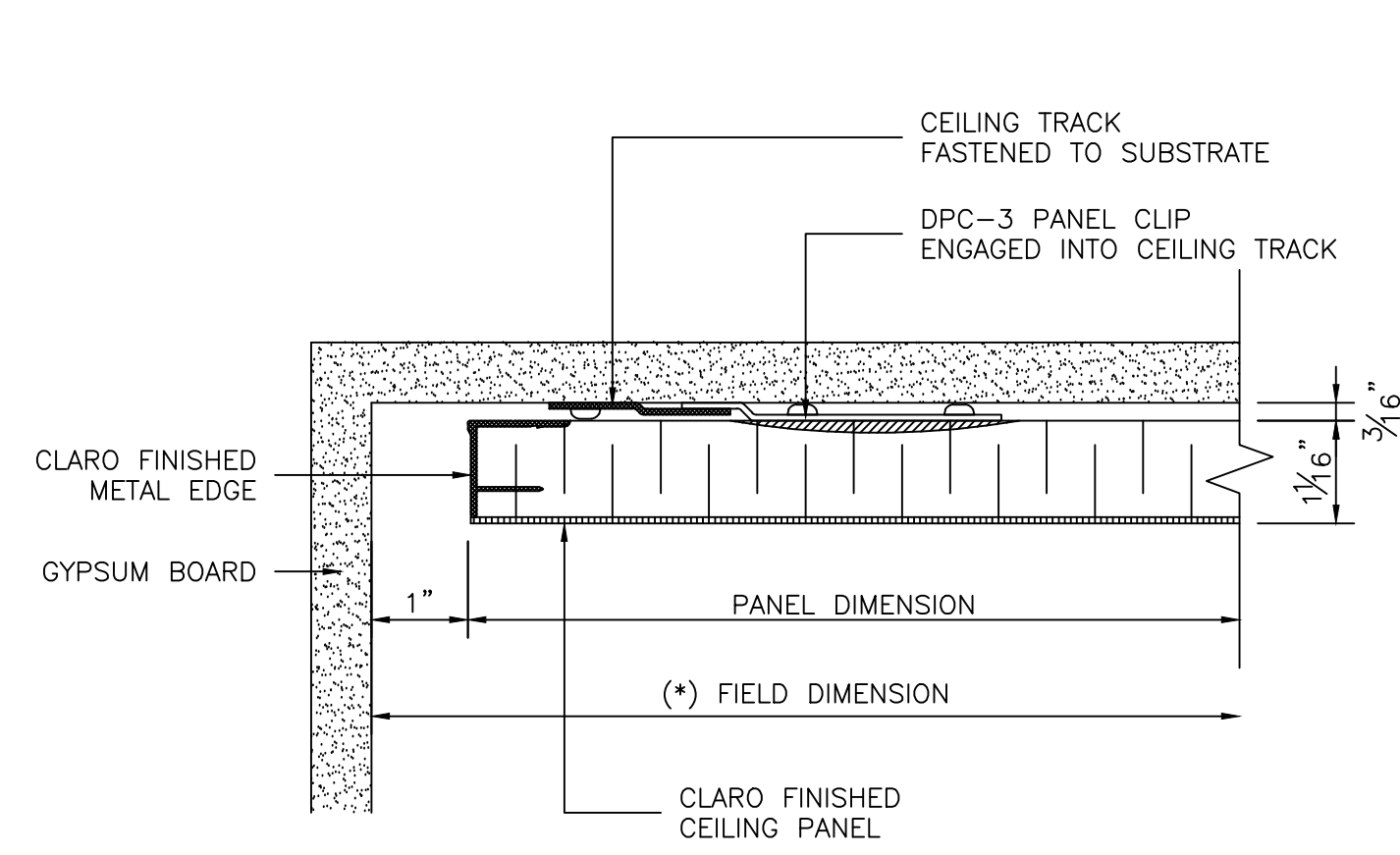
1 FIRST PANEL INSTALLED D1 SCALE: 1/2"=1"
