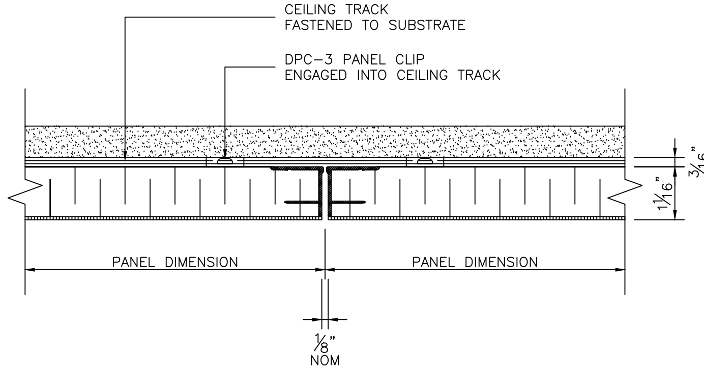
6 PANEL JOINT DETAIL D1 SCALE: 1/2"=1"
