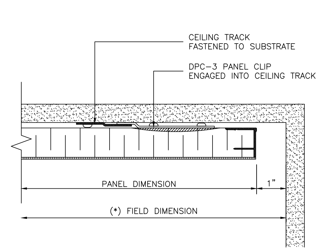
4 LAST PANEL INSTALLED D1 SCALE: 1/2"=1"
