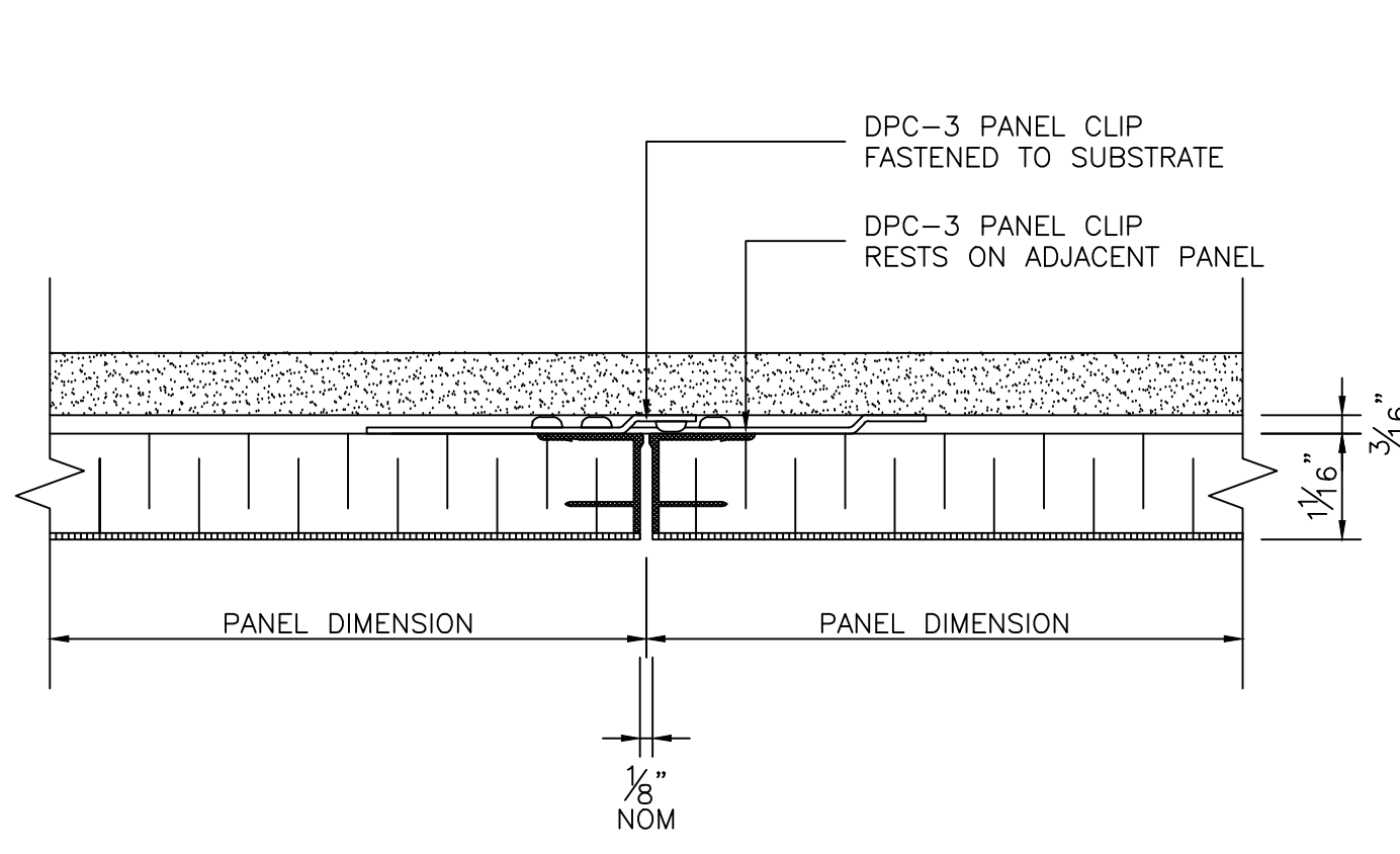
2 PANEL JOINT DETAIL D1 SCALE: 1/2"=1"
