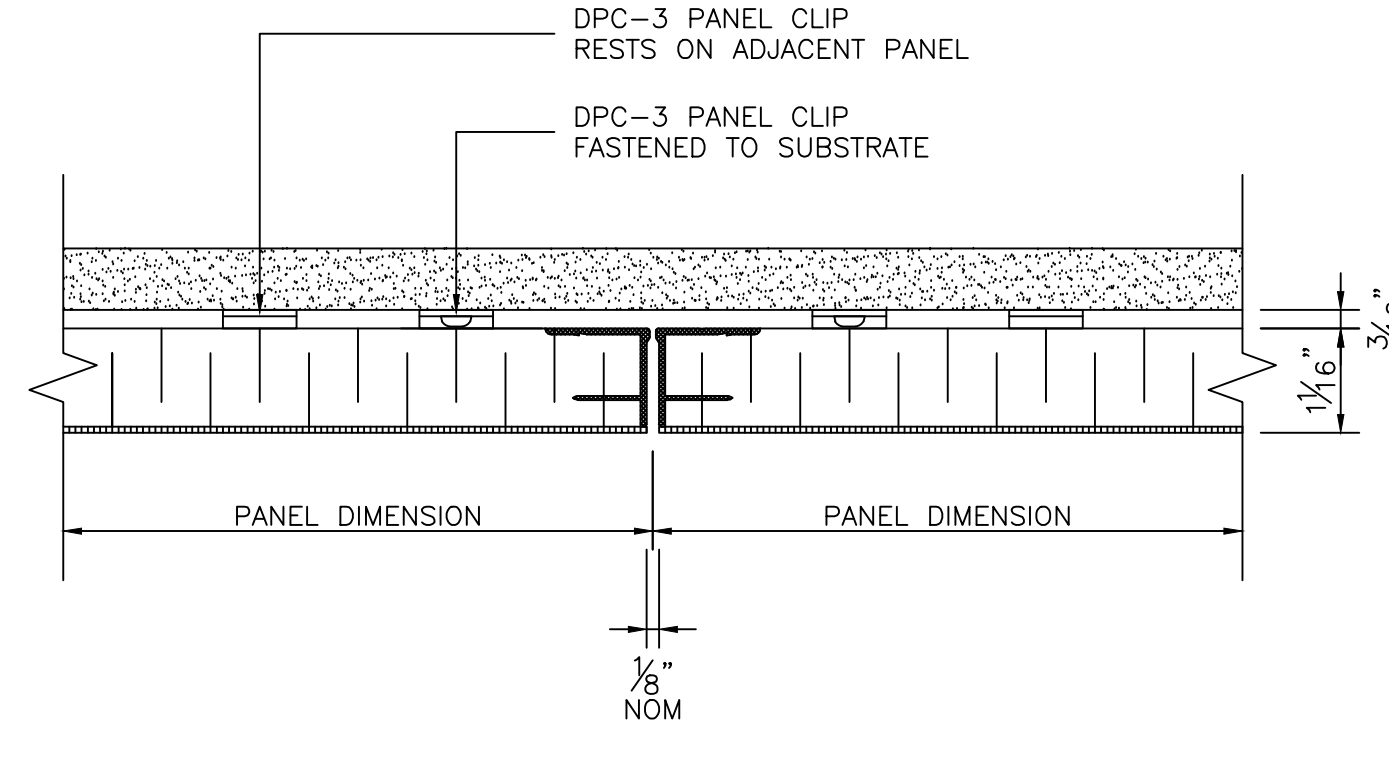
7 PANEL JOINT DETAIL D1 SCALE: 1/2"=1"
