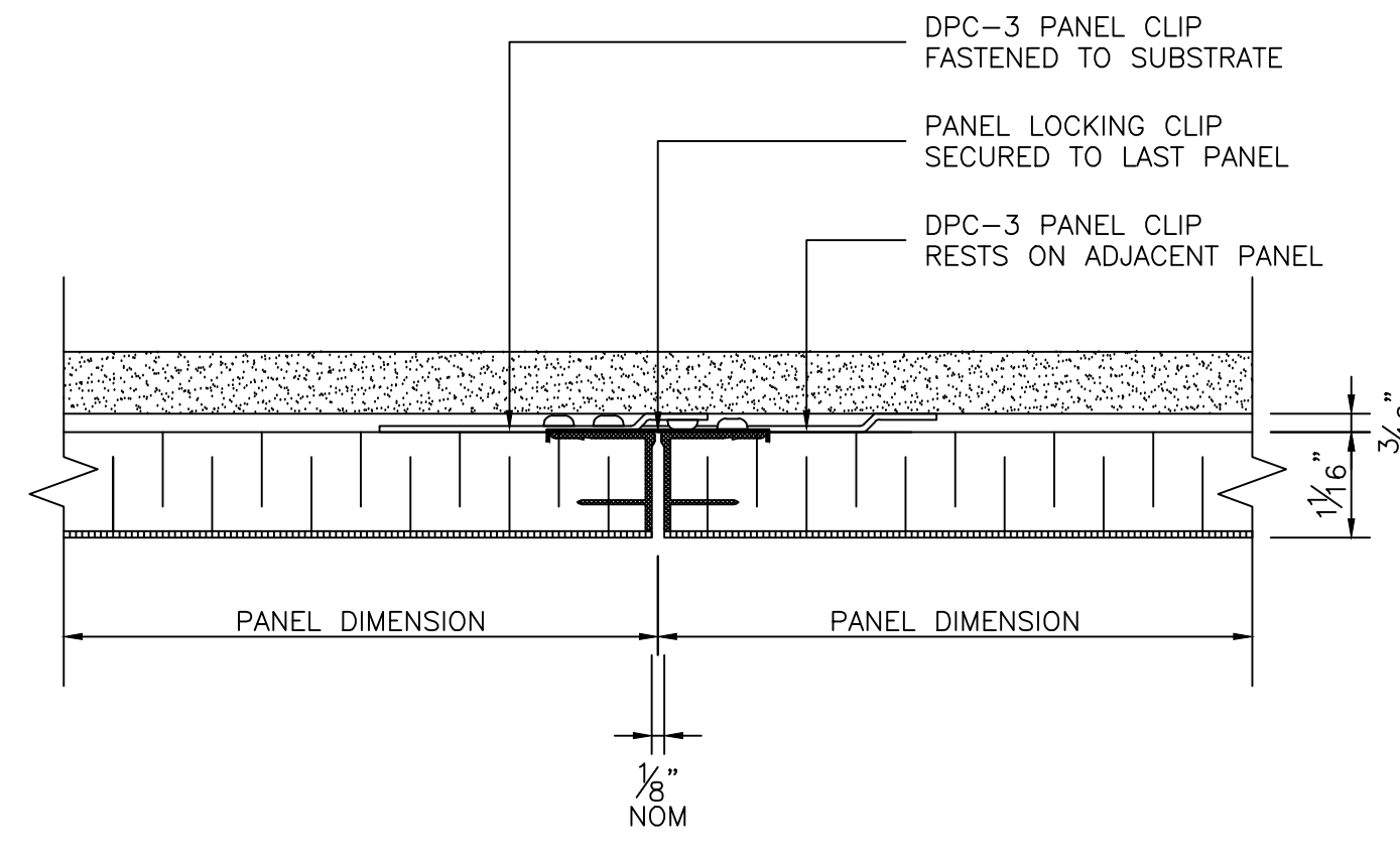
3 PANEL JOINT DETAIL D1 SCALE: 1/2"=1"
