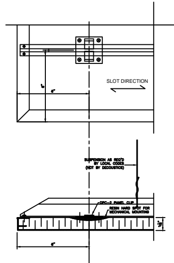
SUSPENDED REVEAL
