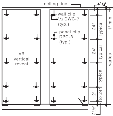
Reveal Arrangement
