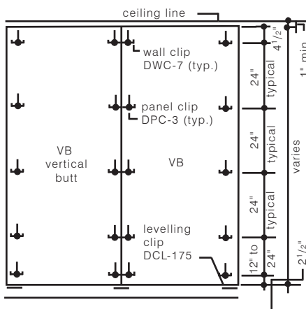
Butt Arrangement
