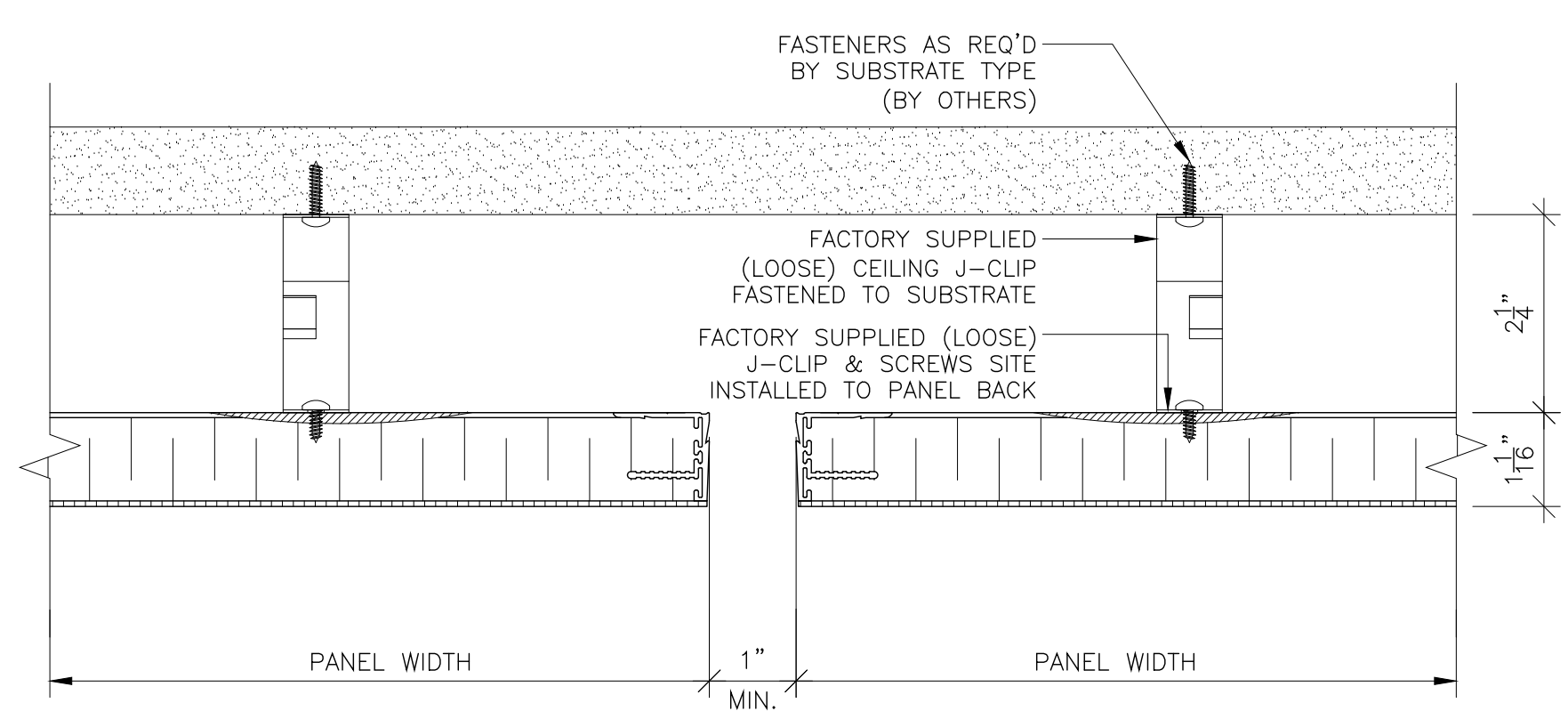
5 PANEL JOINT DETAIL SCALE: 6" = 1'-0"
