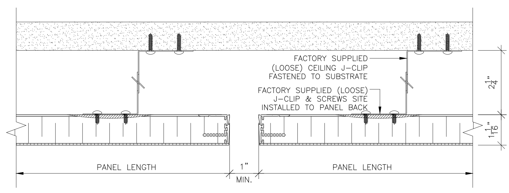
2 PANEL JOINT DETAIL SCALE: 6" = 1'-0"
