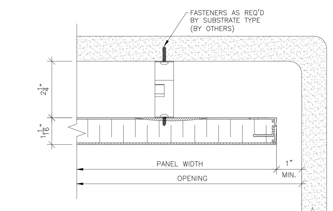
6 PERIMETER PANEL DETAIL SCALE: 6" = 1'-0"
