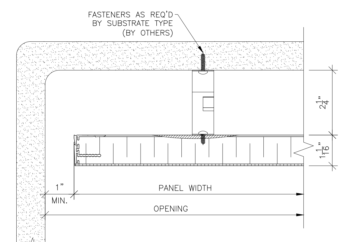
4 PERIMETER PANEL DETAIL SCALE: 6" = 1'-0"
