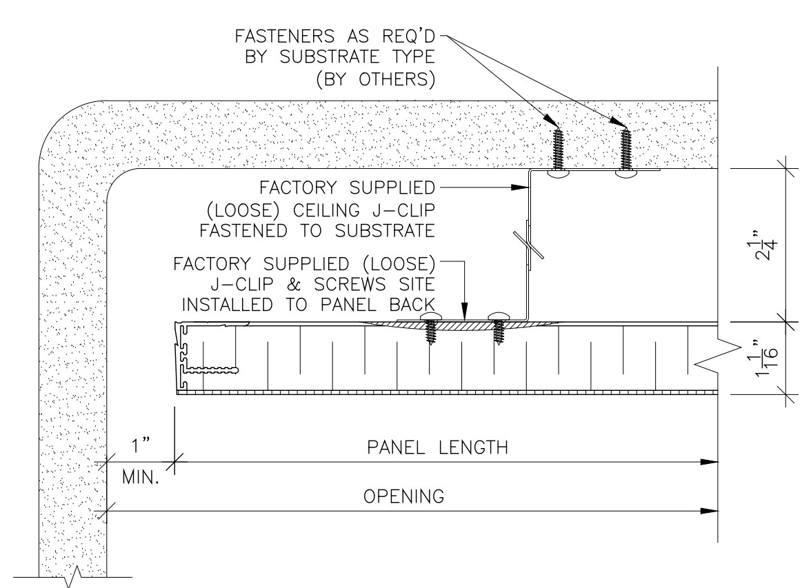
1 PERIMETER PANEL DETAIL SCALE: 6" = 1'-0"
