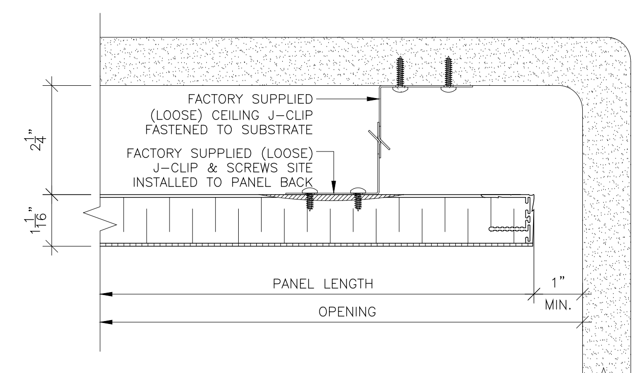
3 PERIMETER PANEL DETAIL SCALE: 6" = 1'-0"
