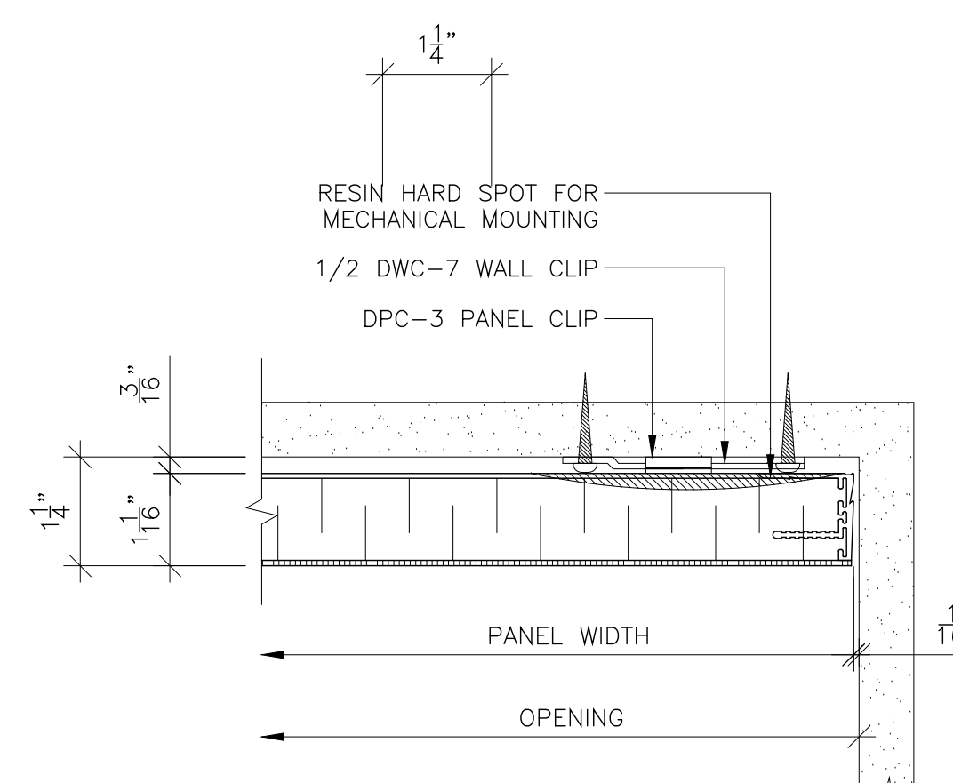
7 PANEL END @ WALL SCALE: 6" = 1'-0" REF:
