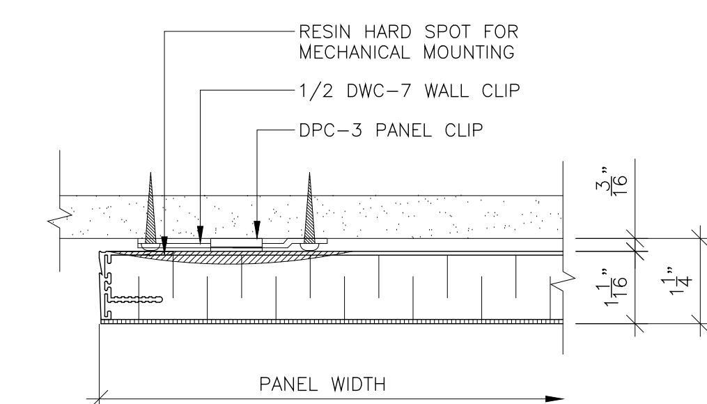
9 PANEL END DETAIL @ WALL SCALE: 6" = 1'-0" REF:
