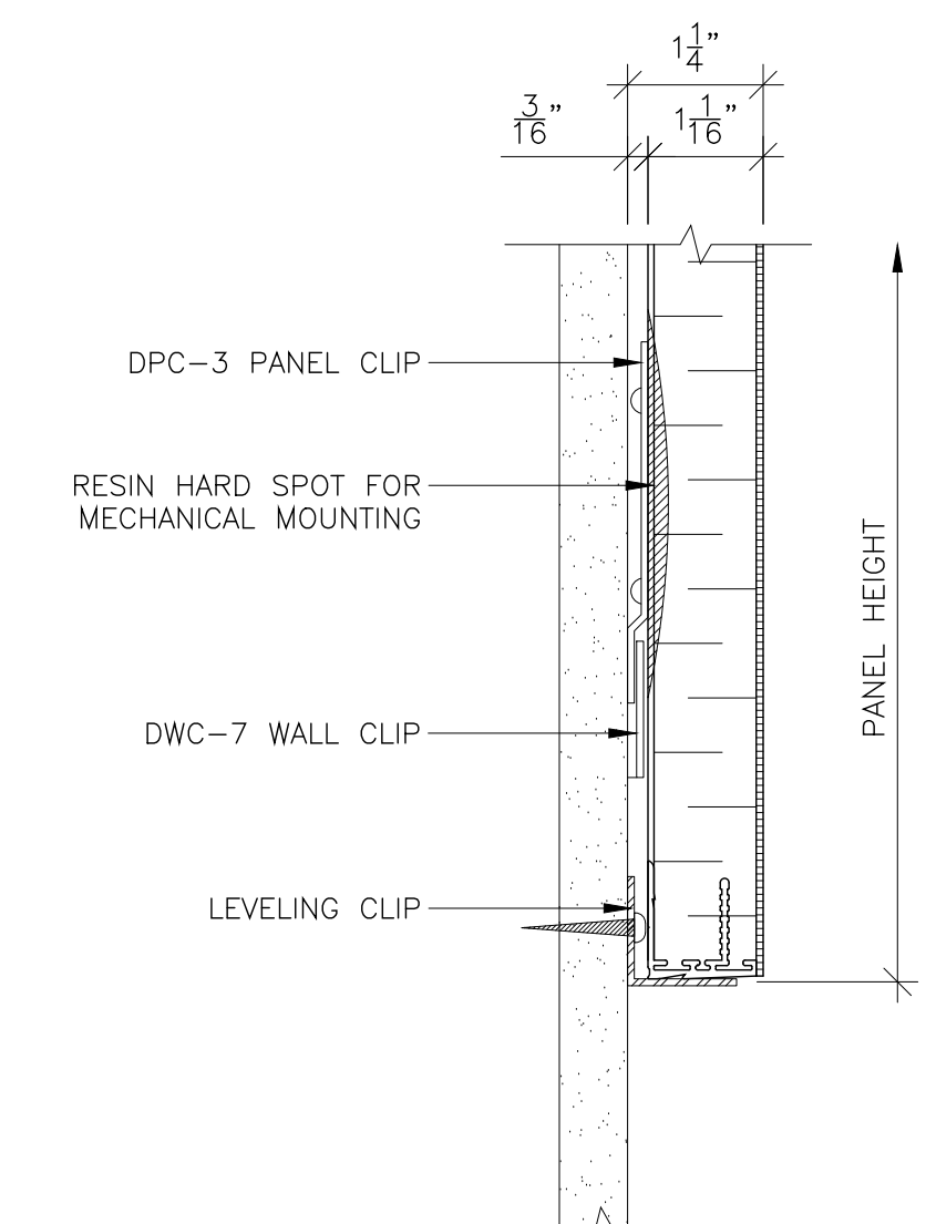
5 PANEL BASE @ WALL SCALE: 6" = 1'-0" REF:
