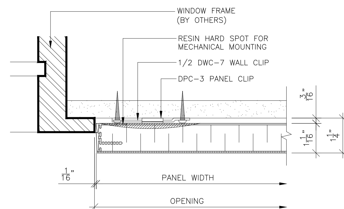
10 PANEL END DETAIL @ FRAME SCALE: 6" = 1'-0" REF:
