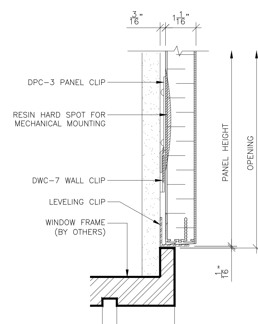
6 PANEL BASE @ FRAME SCALE: 6" = 1'-0" REF:
