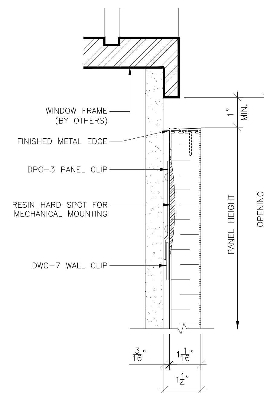
11 PANEL HEAD DETAIL UNDER FRAME SCALE: 6" = 1'-0" REF:
