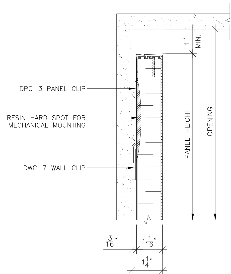
1 PANEL HEAD @ BULKHEAD SCALE: 6" = 1'-0" REF:
