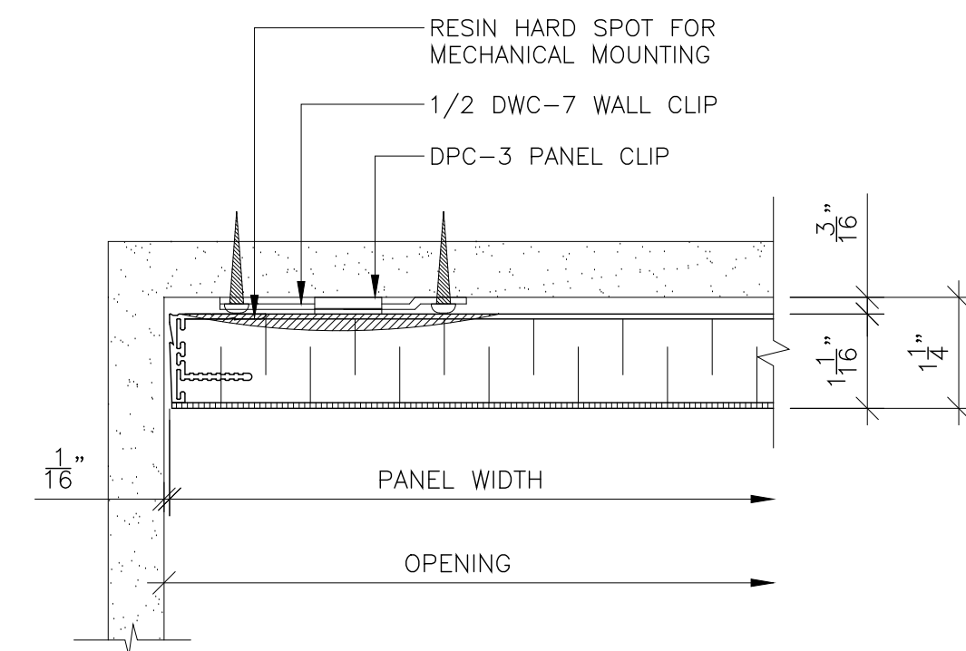
2 PANEL END @ WALL SCALE: 6" = 1'-0" REF:
