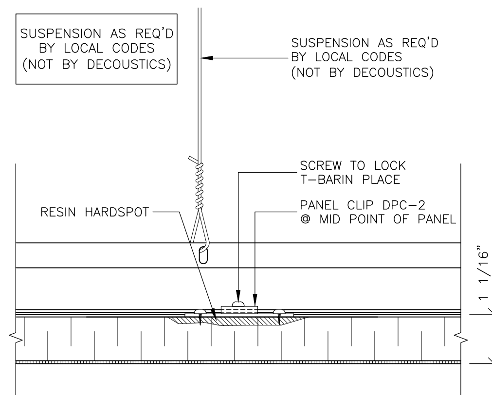
4 CENTER DETAIL (T-BAR FOR PANELS OVER 48" TO 60") D1 SCALE: 6" = 1'-0"
